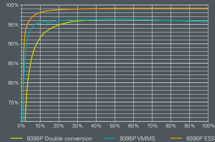
VMMS efficiency is based on system of 10 power modules
